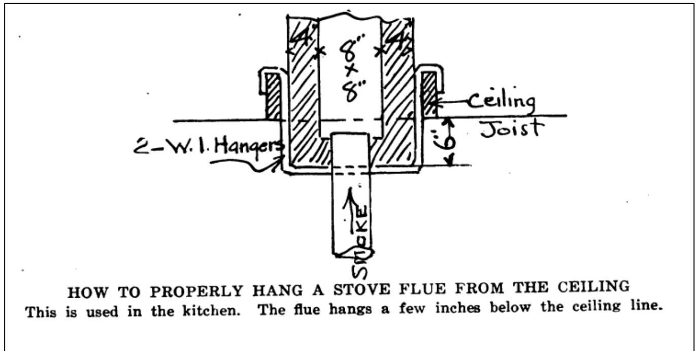
Figure 5. Detail of hung chimney design (Image Source: The Negro Rural School and Its Relation to the Community [Tuskegee, Alabama: The Extension Department, Tuskegee Normal and Industrial Institute, 1915], p. 23.)
